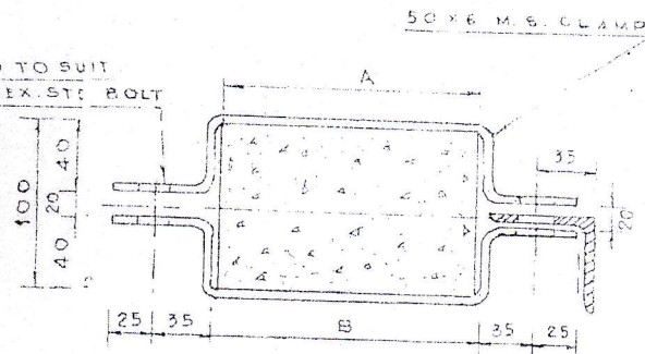
DETAILS OF M.S. CLAMP SCALE: 1:3
